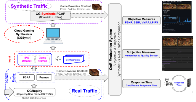
Figure 2: Demonstration setup.
