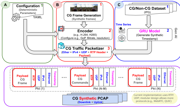
Figure 1: CGSynth architecture modules: (A) System Configuration, (B) Packet Synthesizer, and (C) Synthetic Trace Generator.
